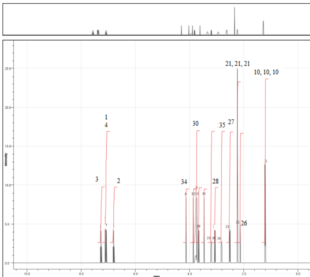
Figure 44: Better resolution of 1 H-NMR spectrum of (AZ-3) by Marvin Sketch.
